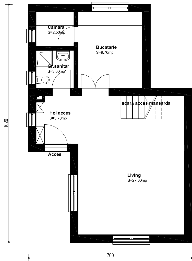
PLAN PARTER
