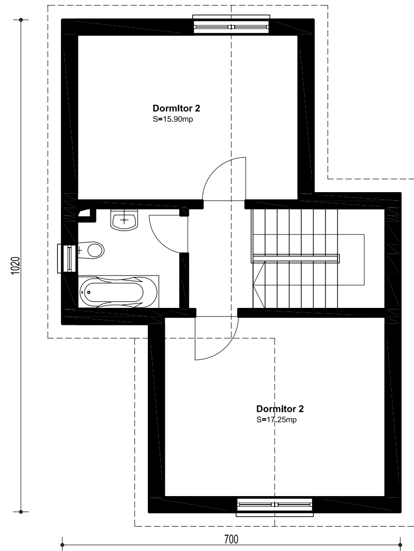
PLAN MANSARDA
